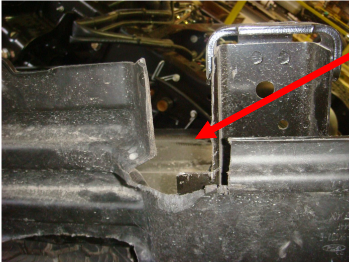
Notch the fuel tank cover so for clearance for the forward trailing arm side mount (drivers side)
