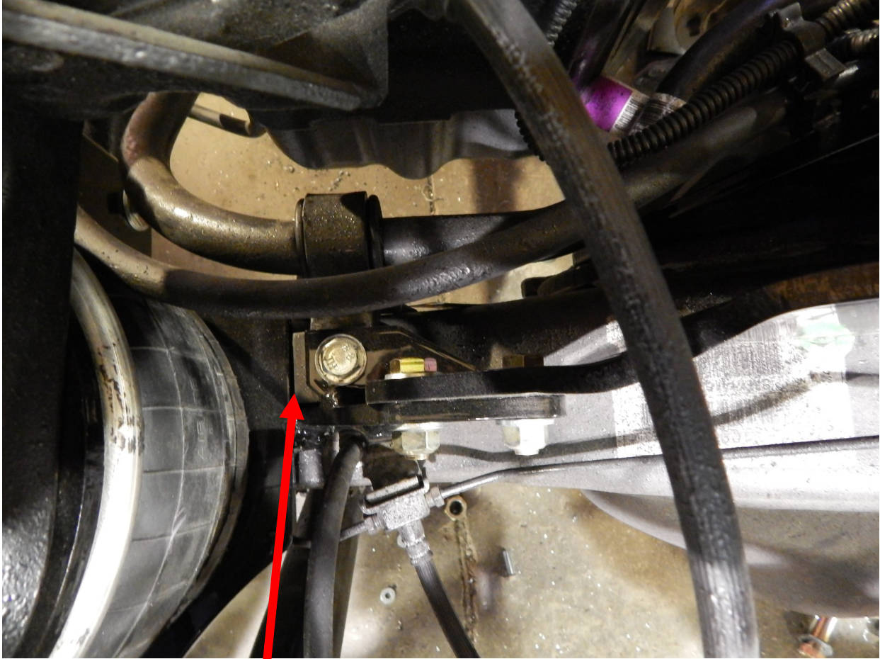
The lower air bag mount will almost be touching the sway bar mounting bracket on the axle
