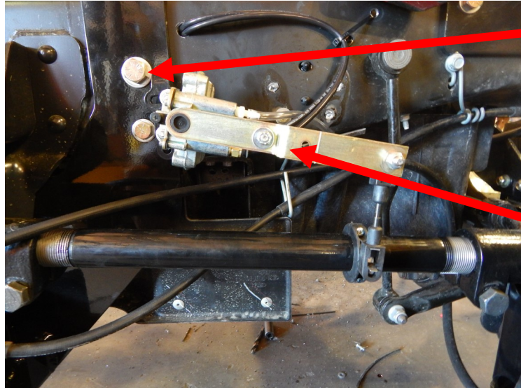
Fine tuning can be done by adjusting the lever once this bolt is loosened.
