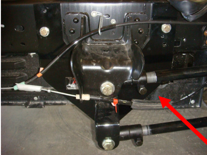
Drivers side forward trailing arm mount installed.
