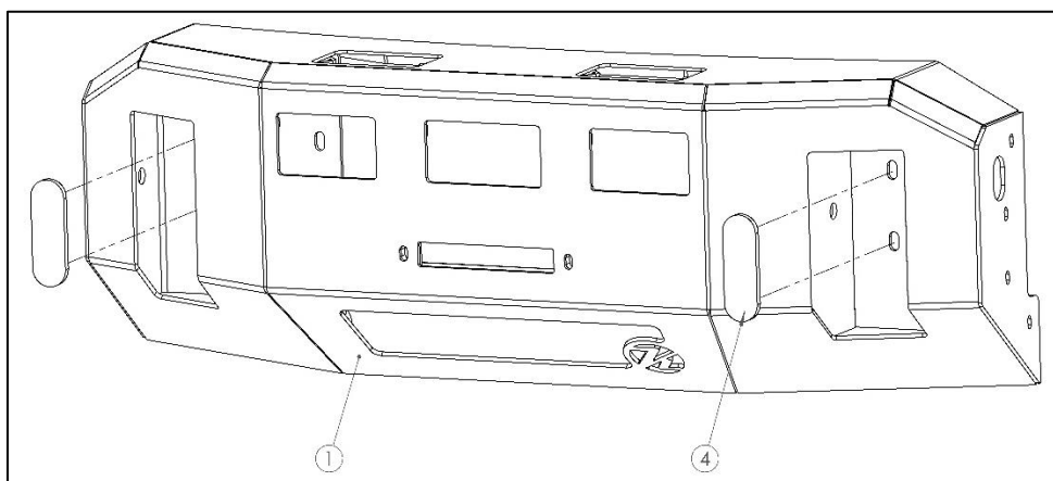
Figure 5: Bolt Tab assembly
