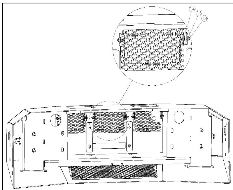
Figure 7: Mesh assembly
