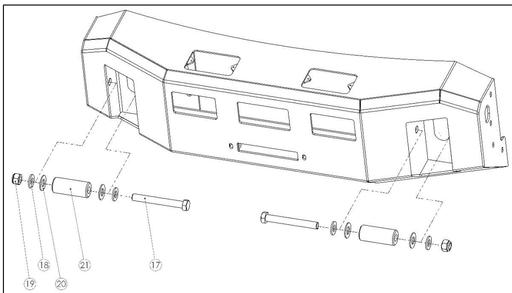
Figure 6: Tow Hook assembly
