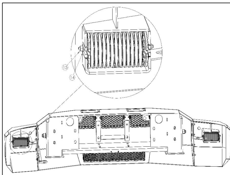
Figure 8: Light assembly
