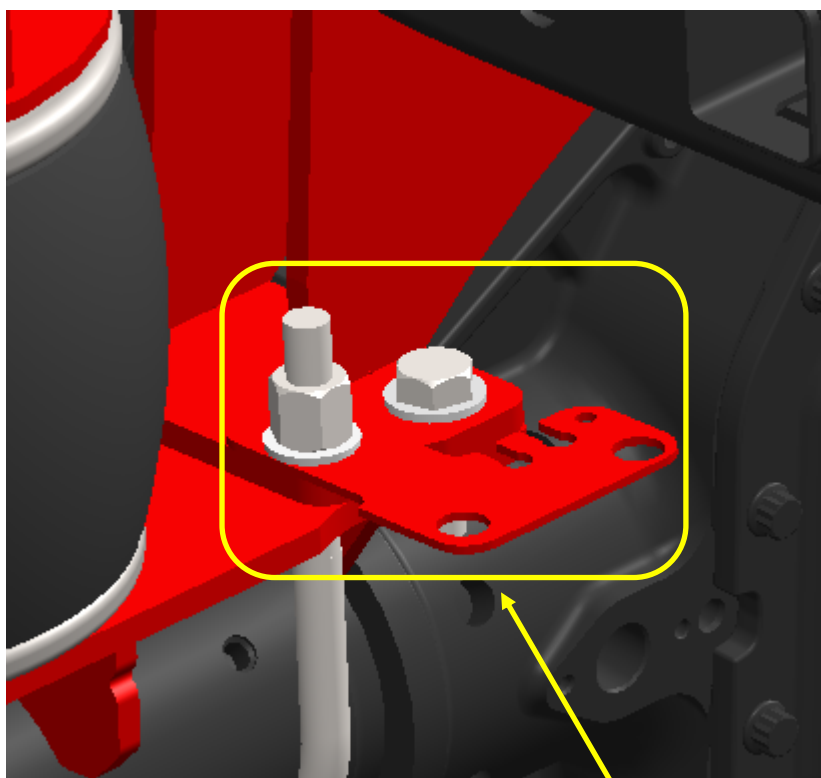
Brake Line Relocation Bracket
