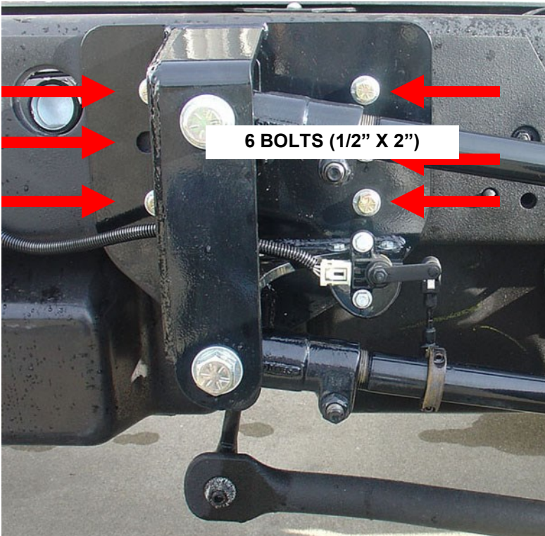
4-LINK SIDE PLATE (DRIVER'S SIDE)
